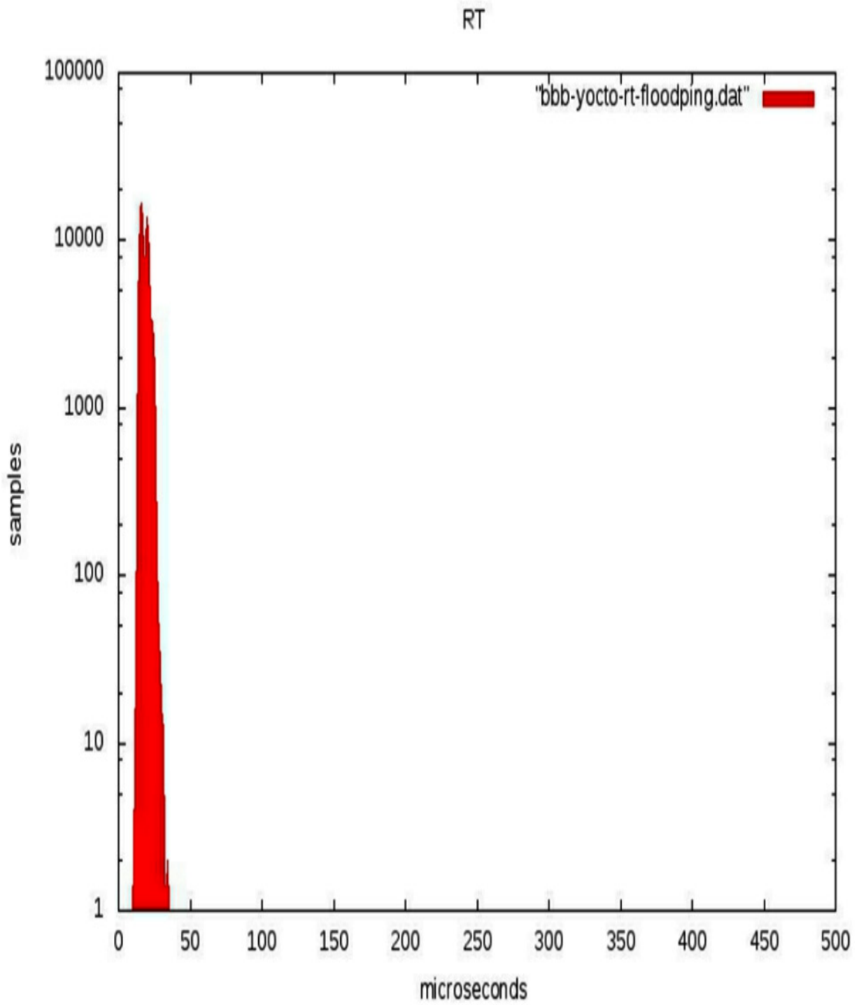
Figure 21.6 – RT preemption
