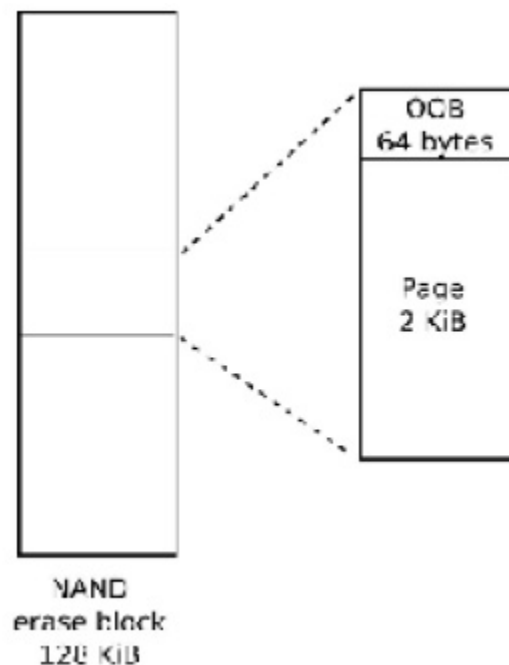
Figure 9.1 – OOB area
