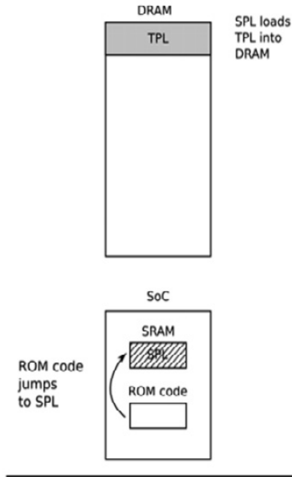
Figure 3.3 – Phase 2 – SPL
