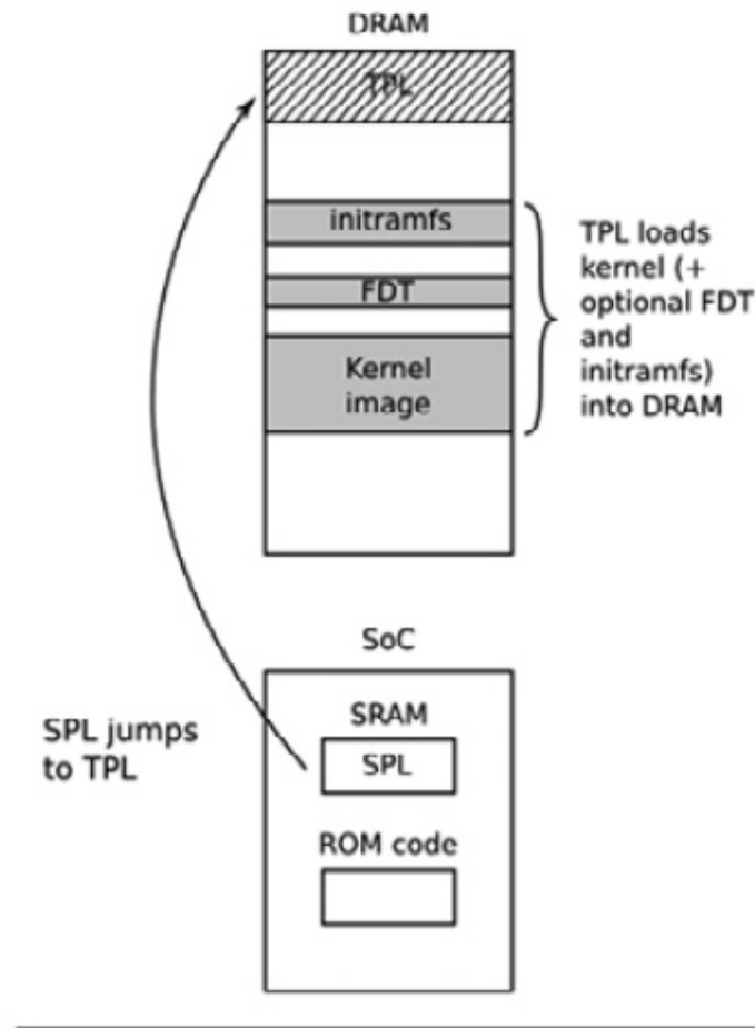
Figure 3.4 – Phase 3 – TPL
