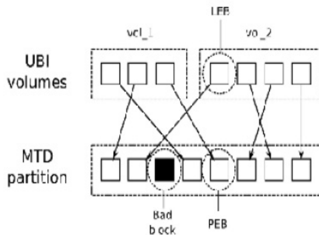
Figure 9.4 – UBI volumes
