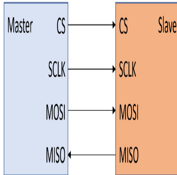
Figure 12.4 – SPI signals
