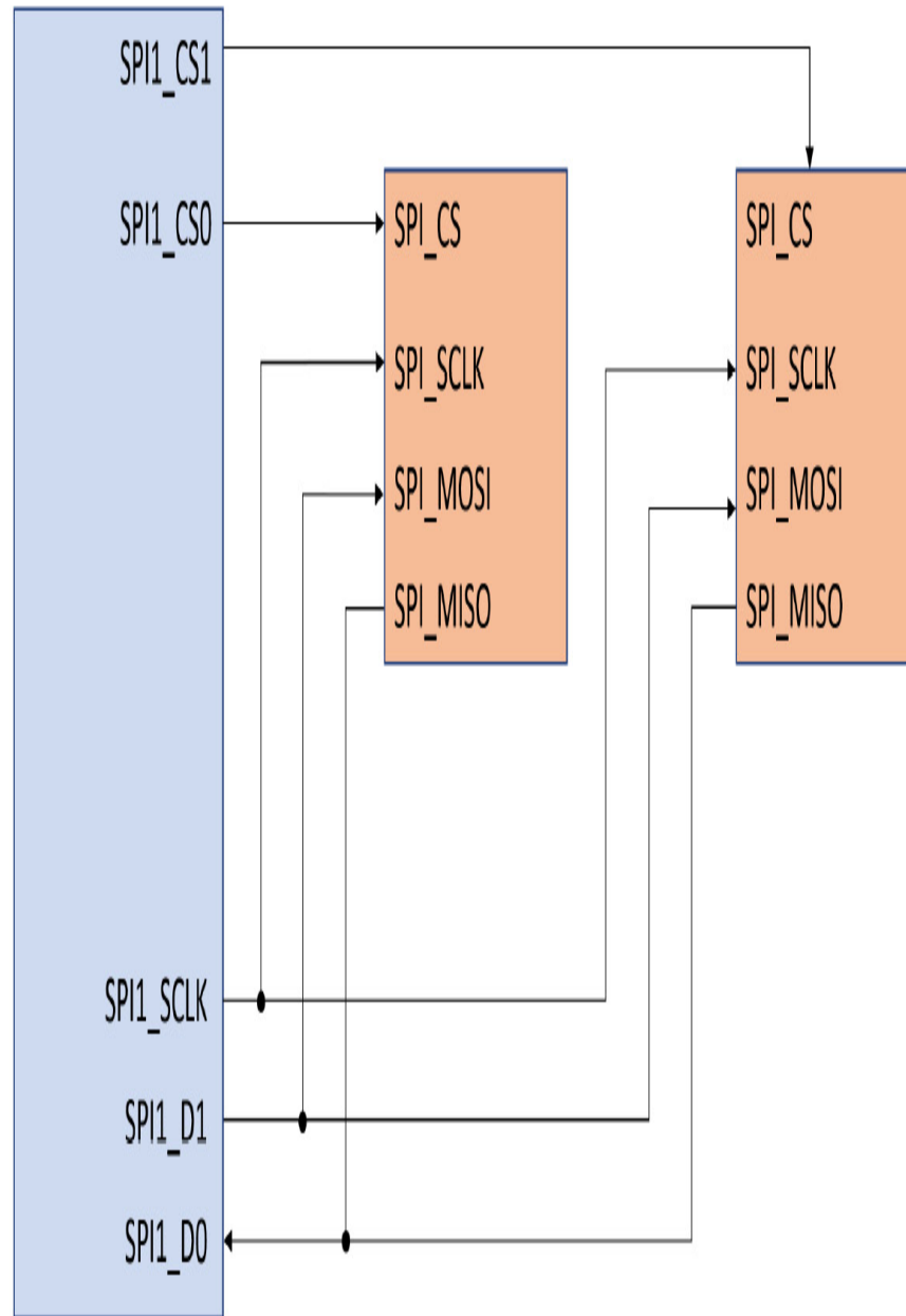
Figure 12.2 – SPI1 bus
