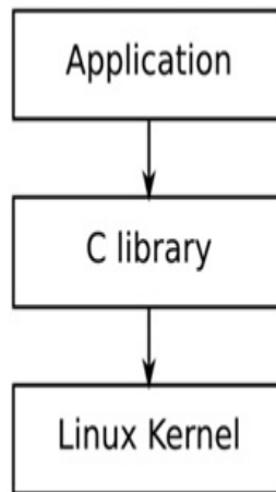
Figure 2.1 – C library
