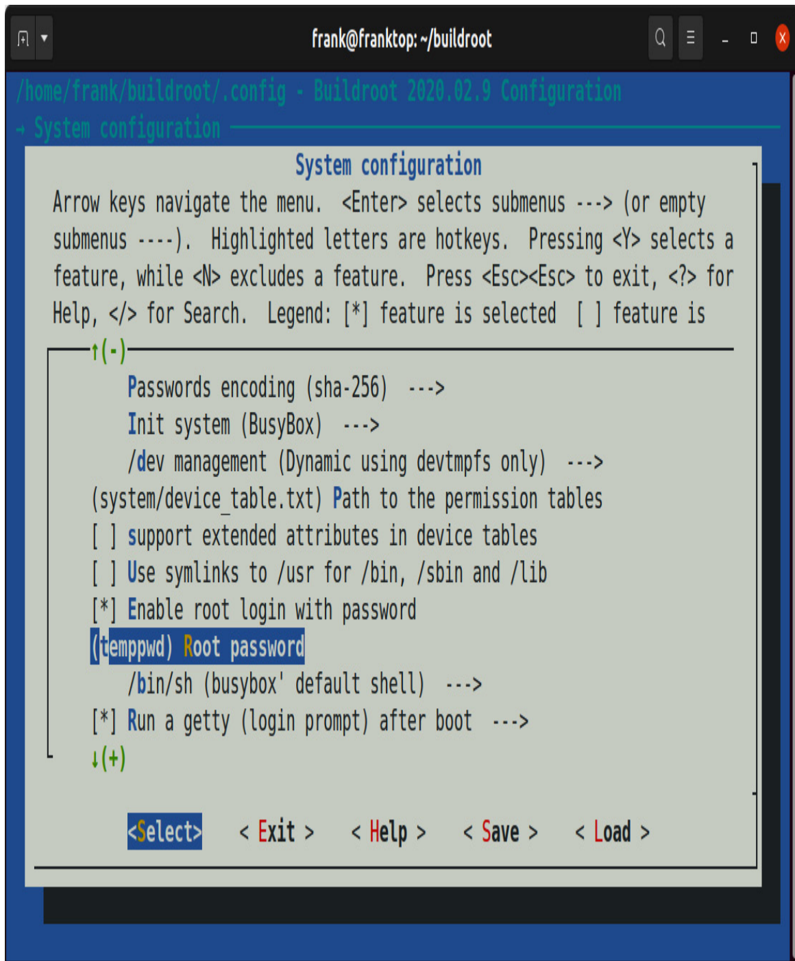
Figure 19.2 – Root password
