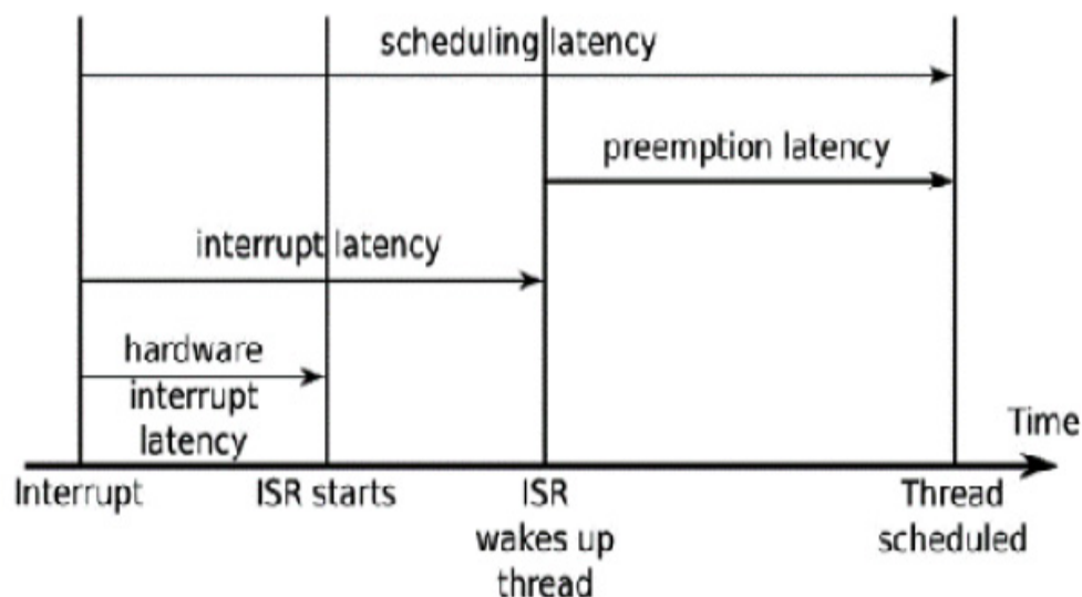
Figure 21.1 – Scheduling latency
