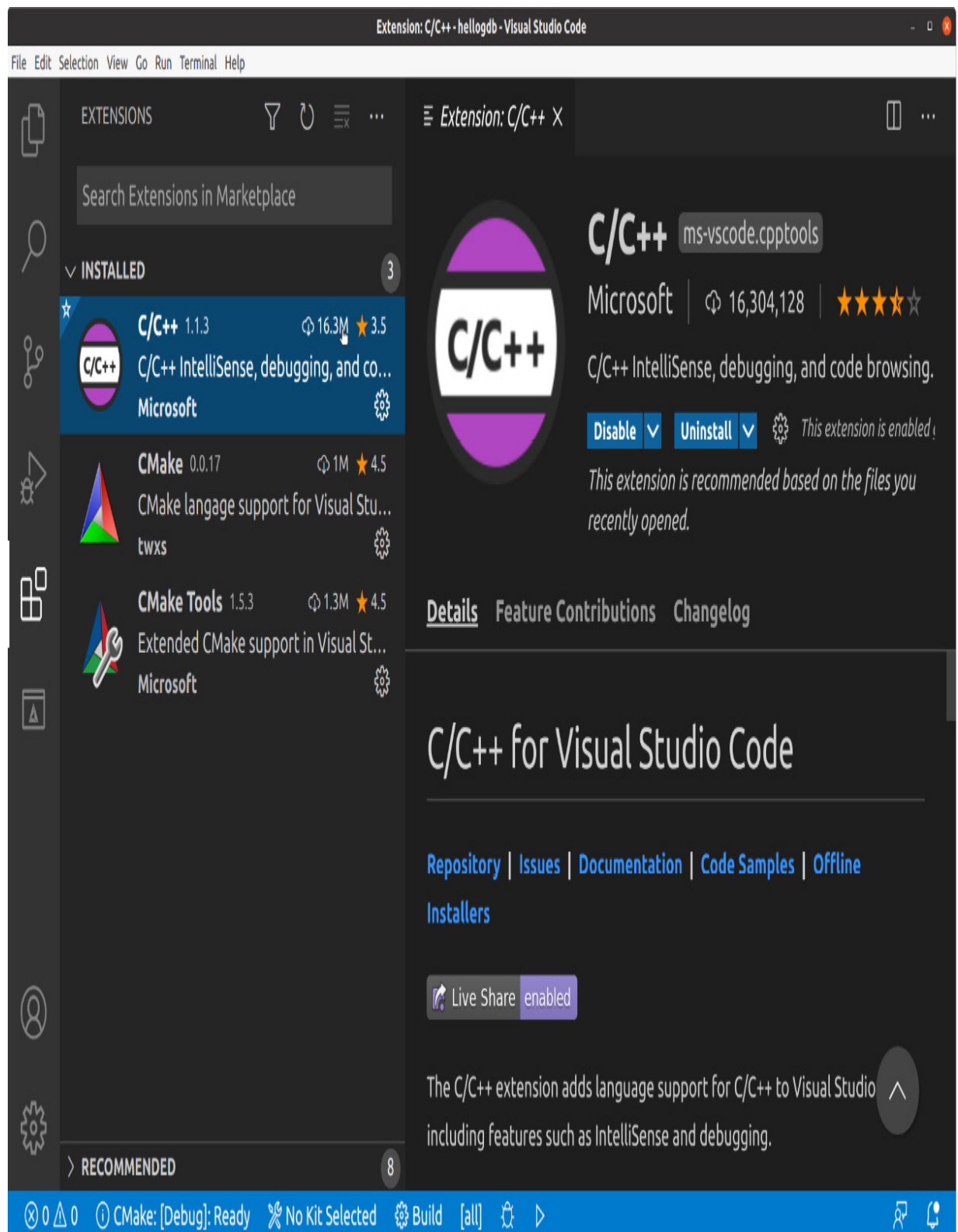
Figure 19.5 – Extensions
