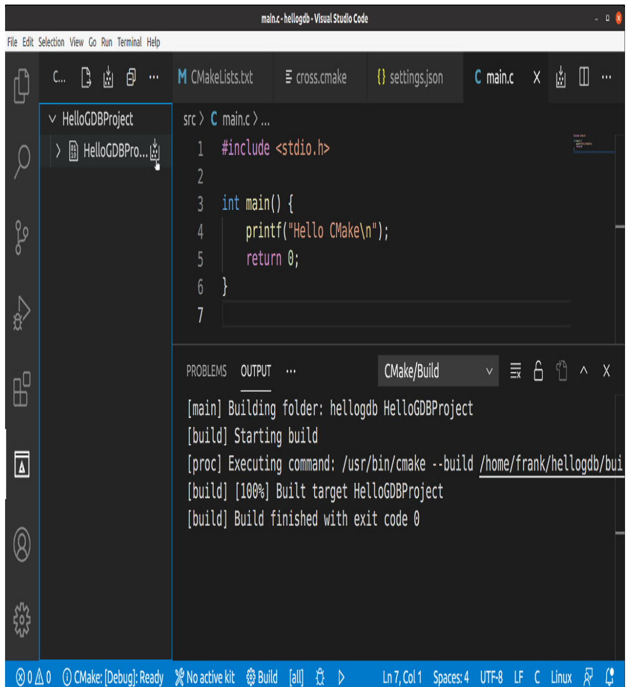
Figure 19.6 – Building HelloGDBProject
