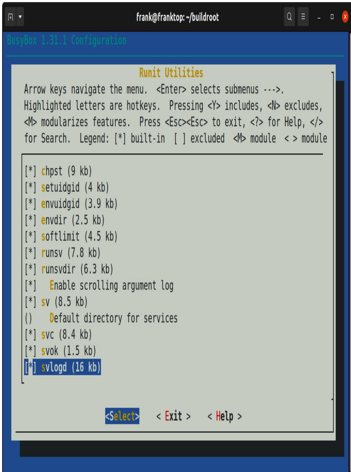
Figure 14.5 – Runit Utilities
