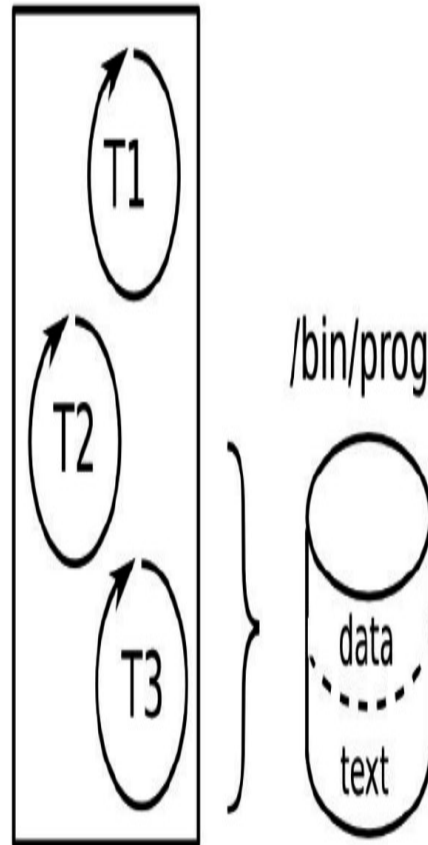
Figure 17.2 – Multiple threads
