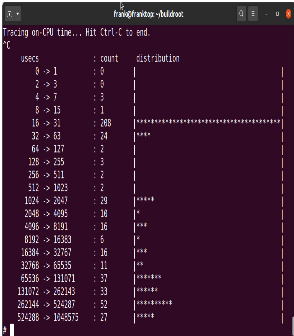
Figure 20.5 – cpudist
