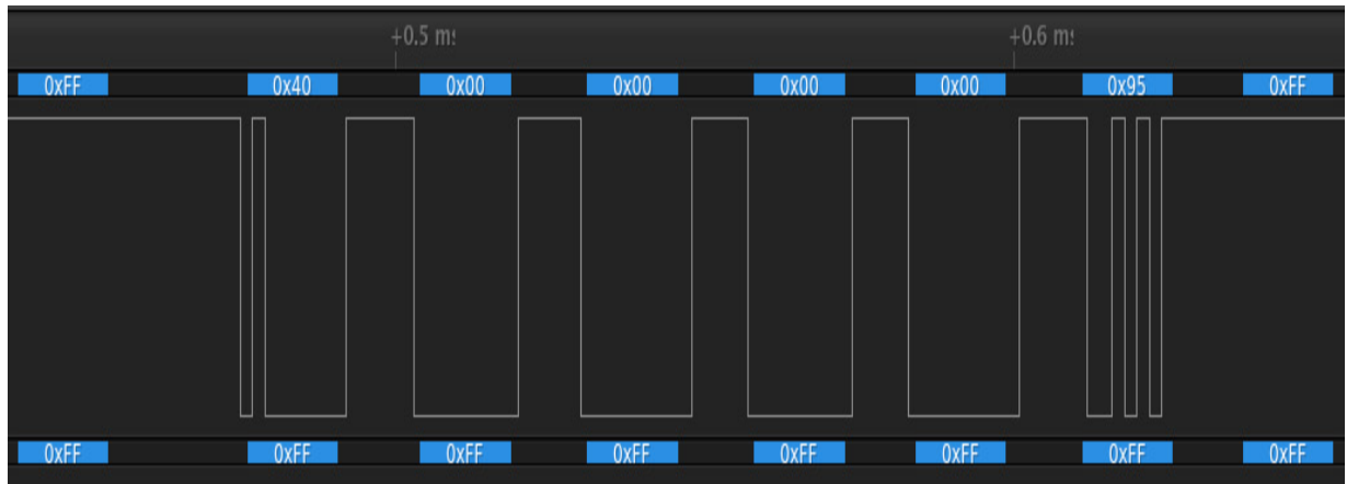
Figure 12.25 – MOSI segment
