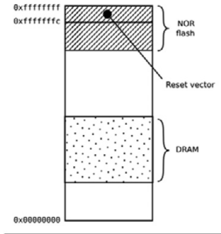
Figure 3.1 – NOR flash
