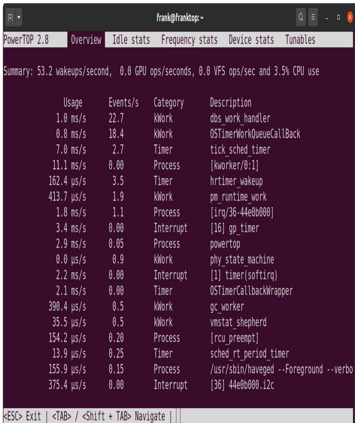
Figure 15.1 – PowerTOP overview
