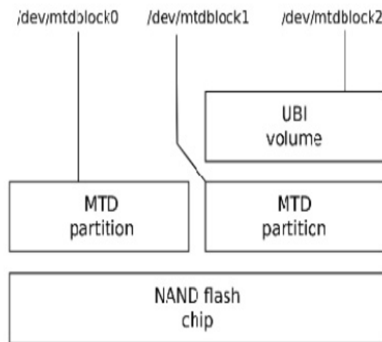
Figure 9.5 – UBI volume
