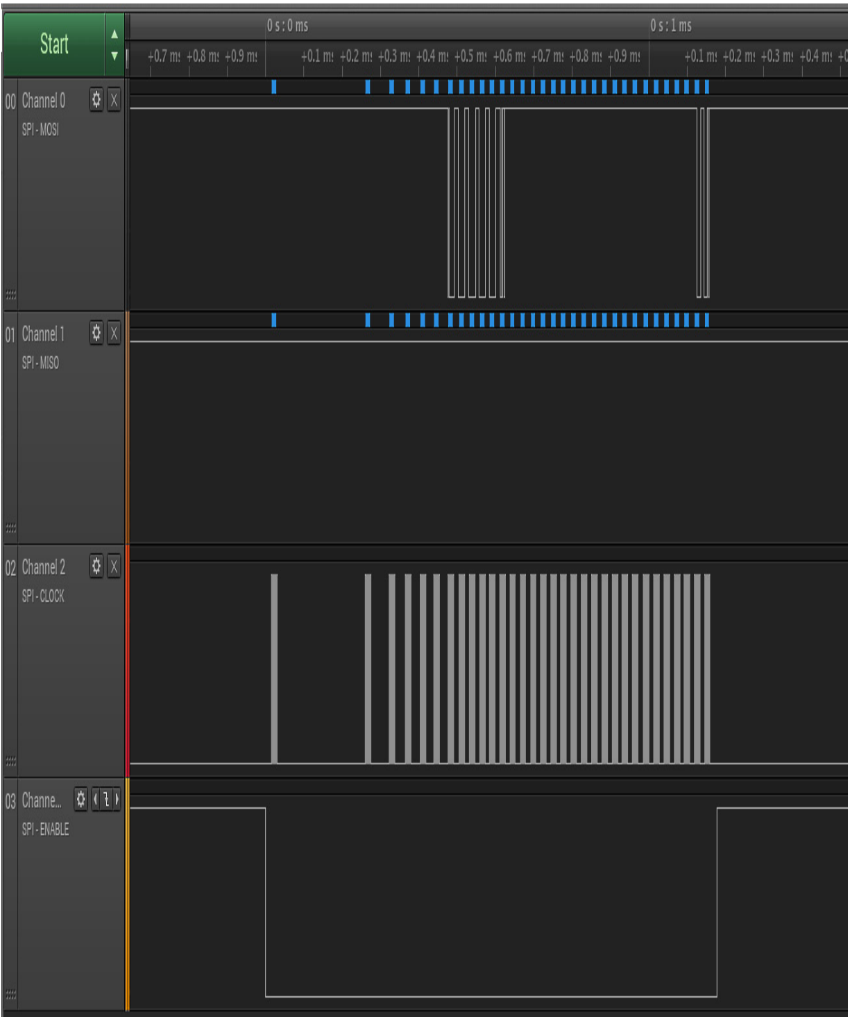
Figure 12.24 – spidev_test transmission
