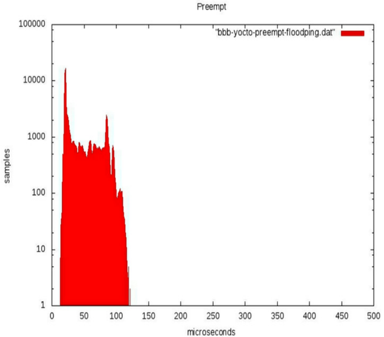
Figure 21.5 – Standard preemption
